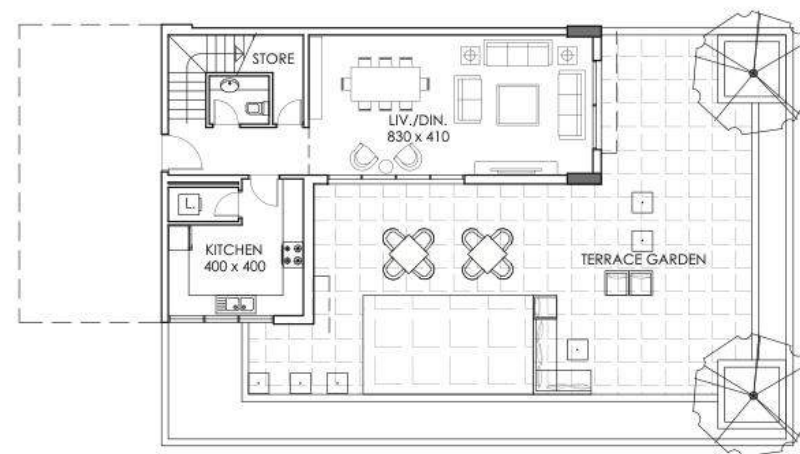
Duplex Lower Level
